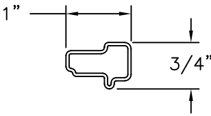
LOCK RAIL/STILE REINFORCEMENT (204A) ALUMINUM 6063-T5
